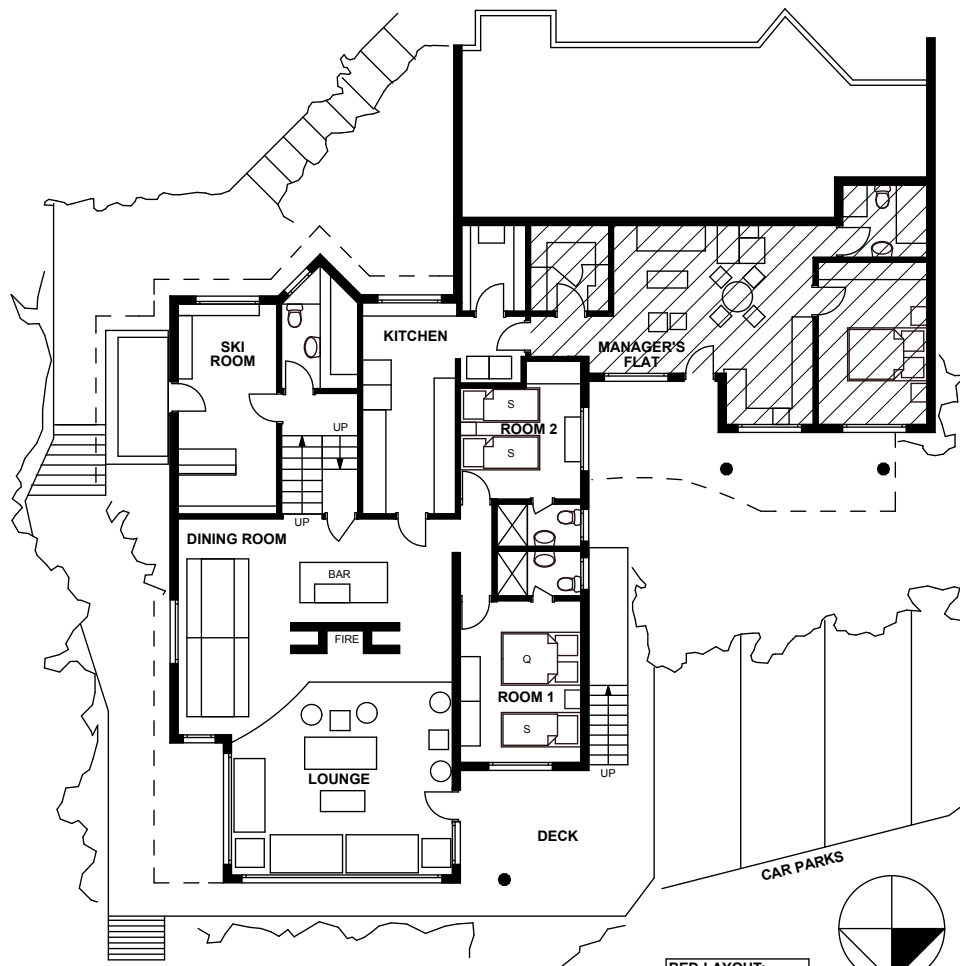
DULMISON THREDBO LOWER FLOOR PLAN
